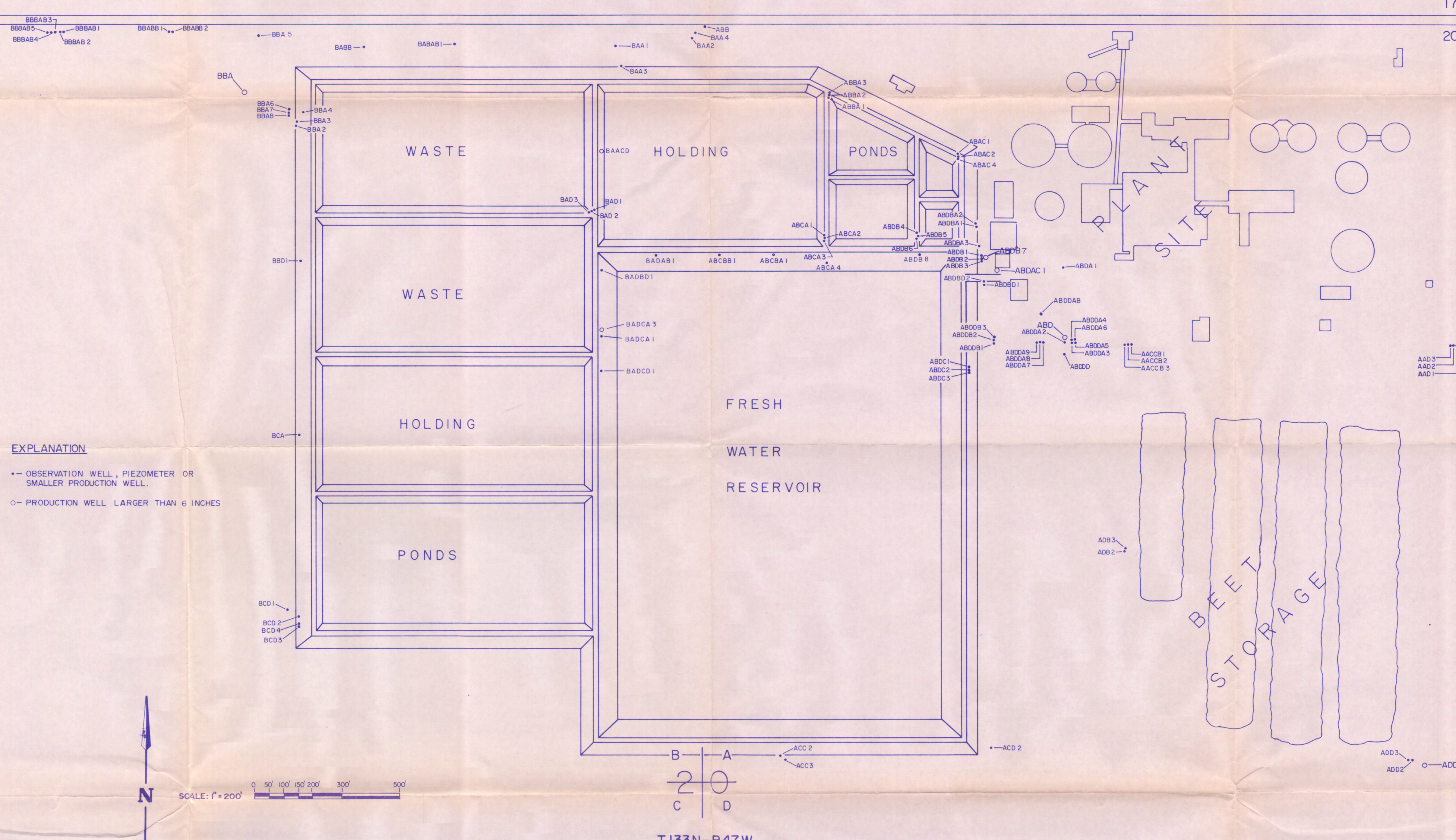
PLATE 2. MAP SHOWING THE LOCATION OF PRODUCTION WELLS, OBSERVATION WELLS, PLANT SITE, BEET STORAGE, RESERVOIR, AND PONDS IN THE N/2 OF SECTION 20 T133N R 47W.
