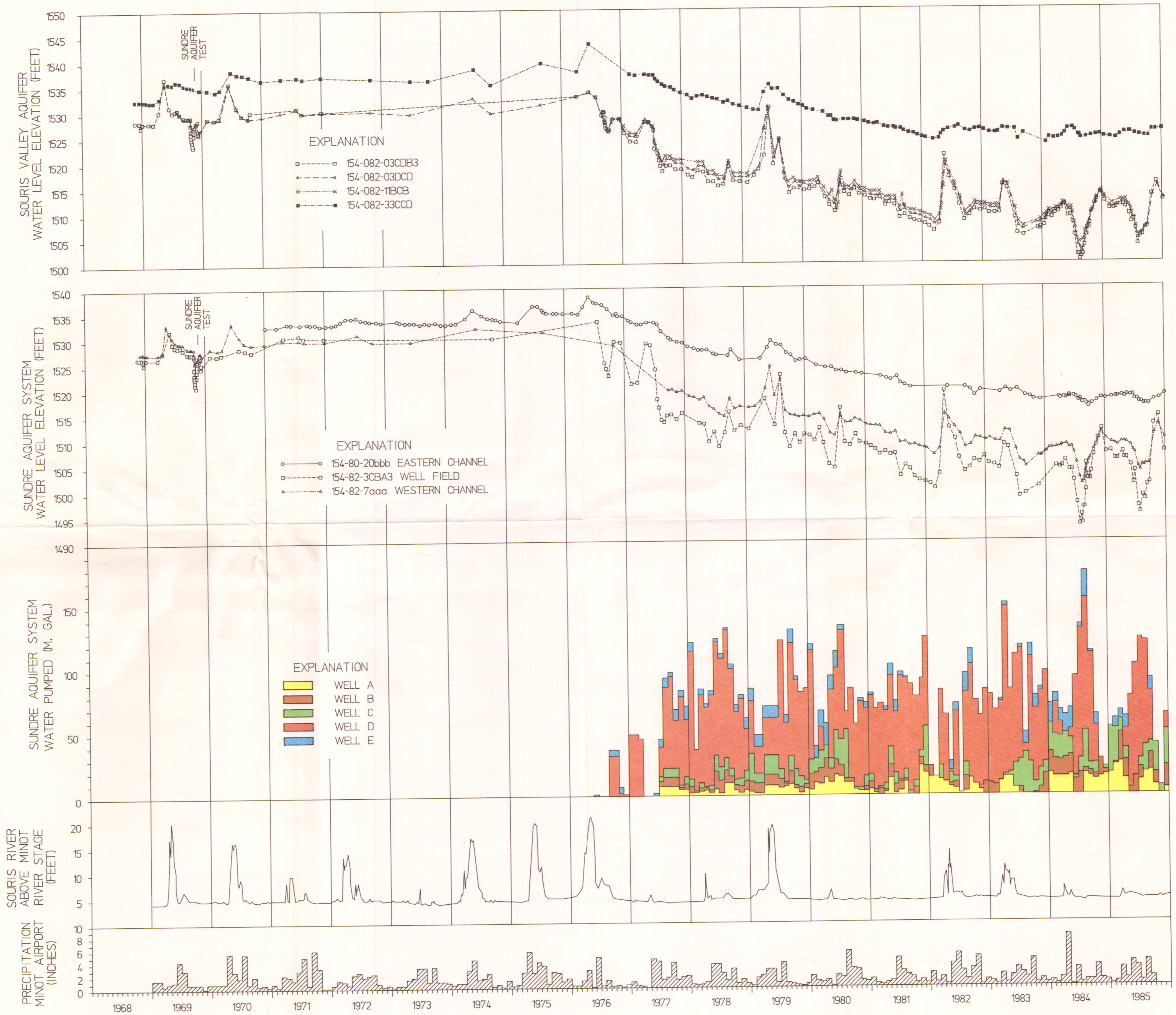
PLATE 2. Comparison of water levels from wells in the Souris Valley Aquifer and Sindre Aquifer versus water use, Souris River stage, and precipitation.
