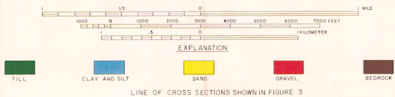
PLATE 3-- GEOLOGIC CROSS SECTIONS IN THE CROSBY AREA
