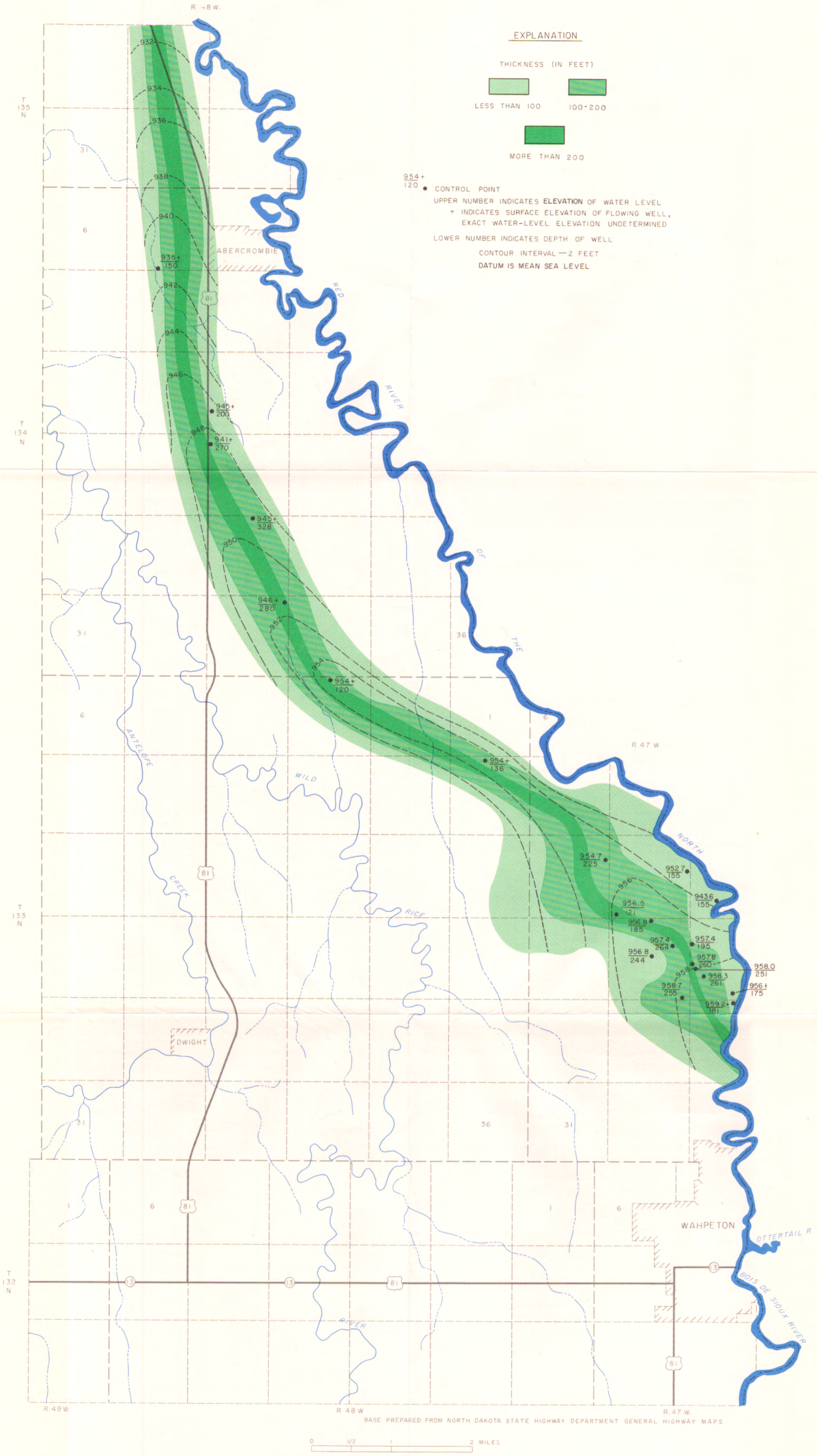
PLATE 5 -- HYDROGEOLOGIC CHARACTERISTICS OF THE WAHPETON BURIED-VALLEY AQUIFER
